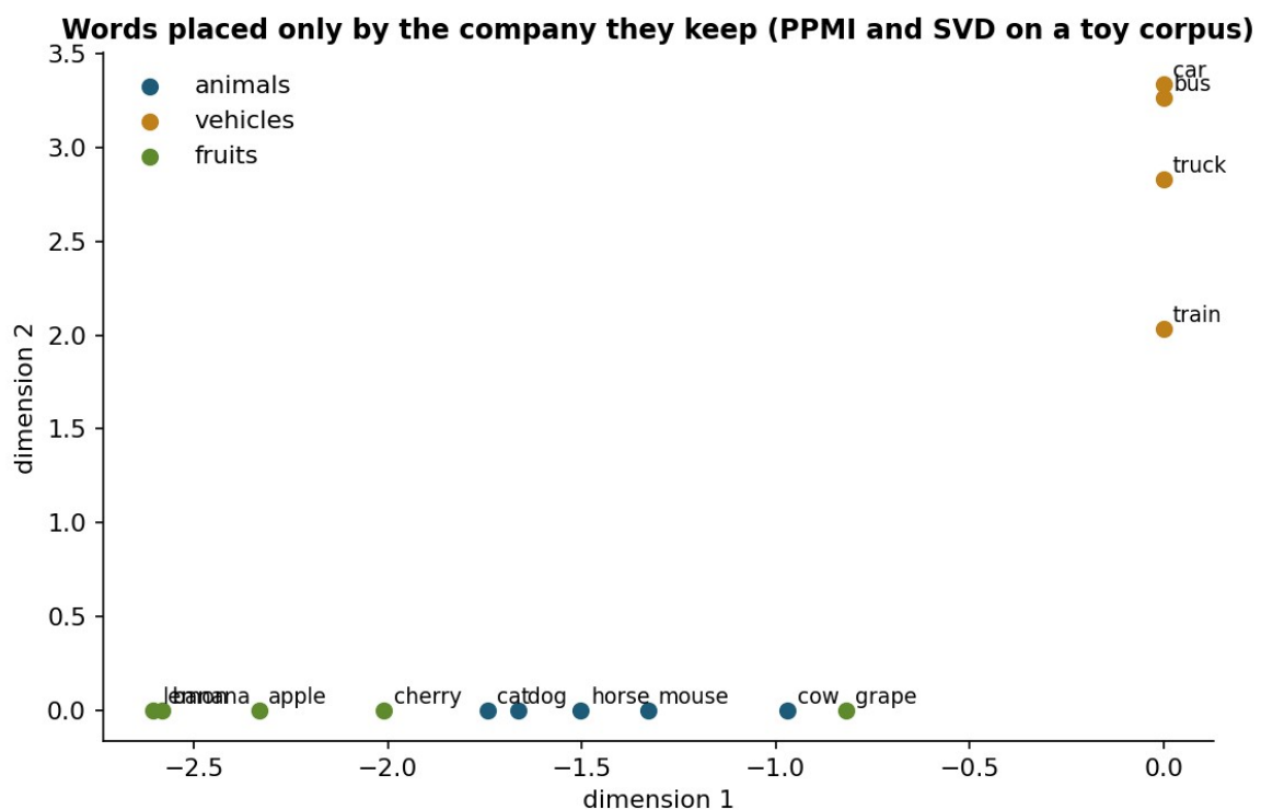
Figure 5.1. Toy corpus words positioned by their co-occurrence statistics alone. The categories separate even though the program has no access to animals, vehicles or fruits [2].
