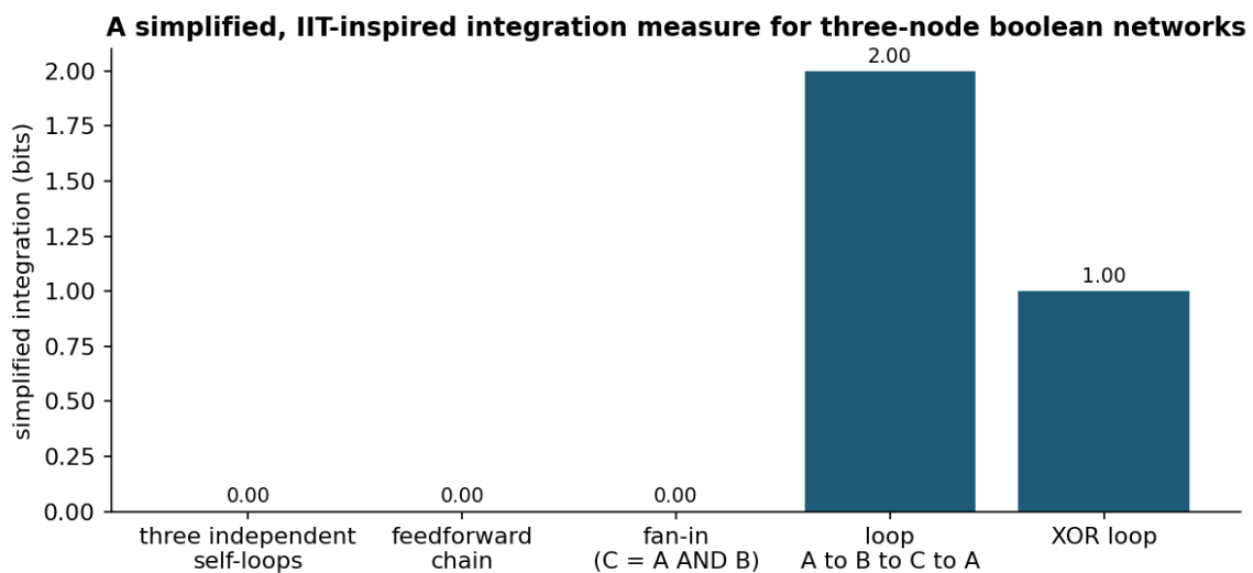
Figure 11.1. A simplified integration measure, whole-system information minus the information of the best split into parts, for five three-node boolean networks. It is inspired by, but not equal to, \Phi of integrated information theory [2, 6].
