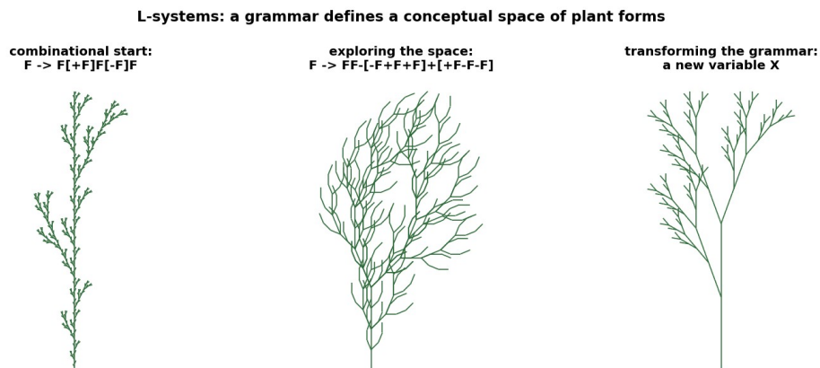
Figure 13.1. Plant forms generated by L-systems. Changing parameters explores the space defined by a grammar, while changing the grammar transforms it [2, 6].
