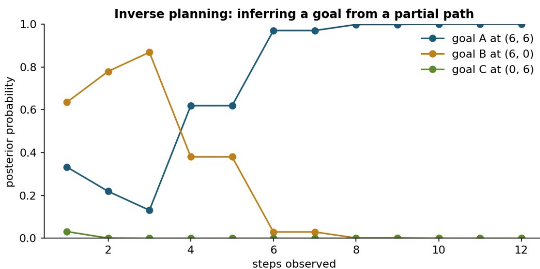
Figure 14.1. Posterior probabilities of three possible goals as successive steps of a path are observed, computed by Bayesian inverse planning [3].
