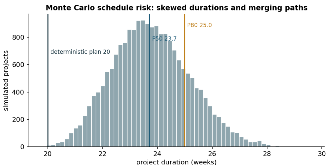
Figure 10.1. Distribution of the duration of the example project in 20,000 Monte Carlo runs with triangular task durations from 0.9 to 1.6 times the planned value [3].
