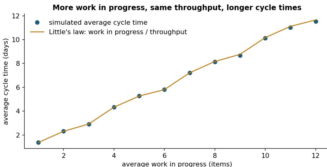
Figure 11.1. Simulated Kanban system with fixed capacity: raising the limit on work in progress leaves throughput unchanged and lengthens cycle times, as Little's law predicts [3].
