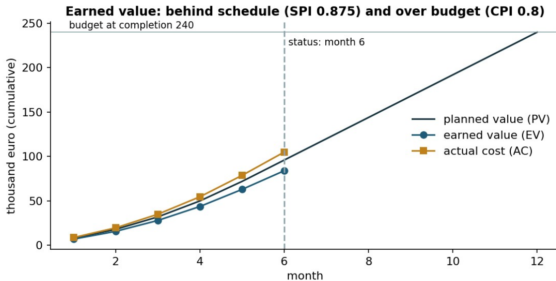
Figure 12.1. Planned value, earned value and actual cost of the example project at month 6 [1].
