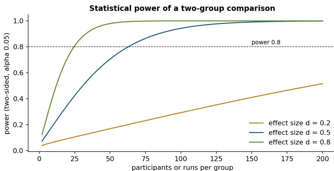
Figure 2.1. Power of a two-sided two-group comparison at a significance level of 0.05 as a function of group size for three effect sizes, computed with a normal approximation.
