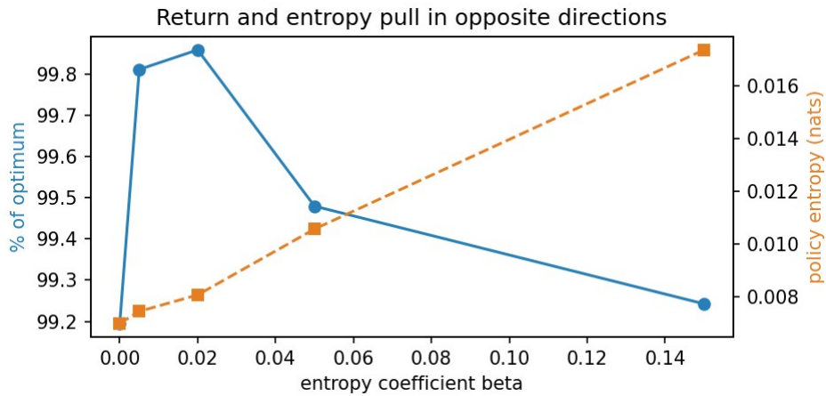
Figure. Return as a percentage of the optimum, left axis, and entropy over the visited states, right axis, against the entropy coefficient \beta , as means over six seeds.
