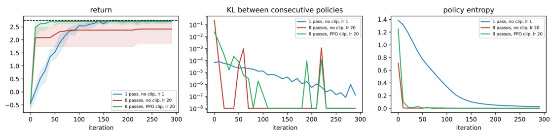
Figure. Return, KL divergence between consecutive policies on a logarithmic scale, and entropy over the visited states, for one pass without the clip and for eight passes without and with it. In the legends, lr is the learning rate.
