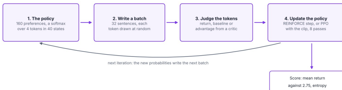
Figure. The learning loop of Day 3 on TokenWorld. The methods differ in step 3, how the tokens of a sentence are judged, and in step 4, how far one batch may move the policy.
