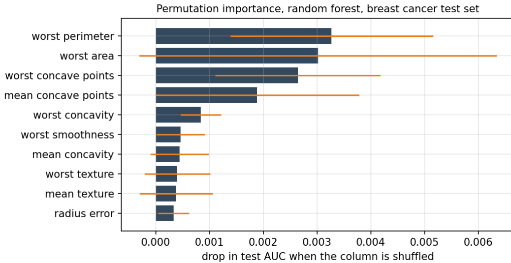
Figure. Permutation importance of the random forest on the test tumours: the mean drop of the test AUC over ten shuffles for the ten most important measurements, with one standard deviation to each side in orange.
