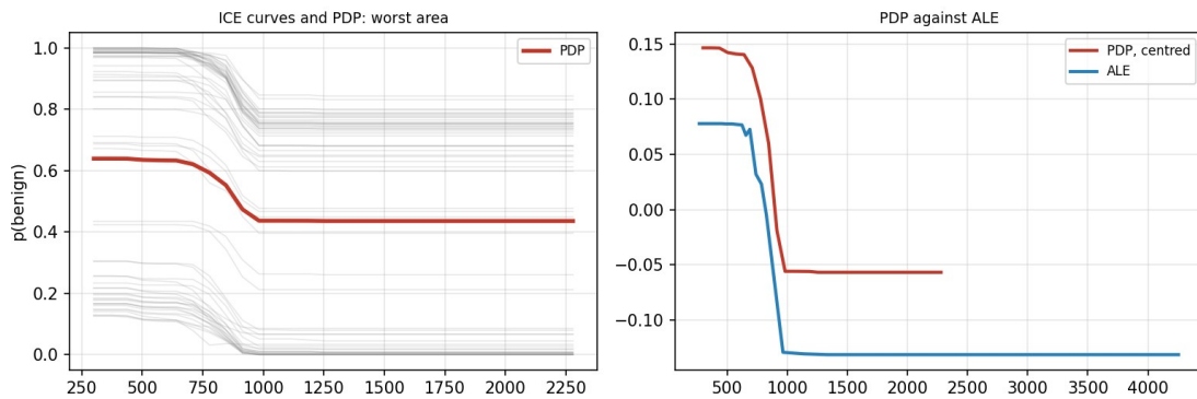
Figure. Left: ICE curves of 60 test tumours and their average, the partial dependence (PDP), for the worst area. Right: the centred partial dependence and the accumulated local effects (ALE) of the same measurement.
