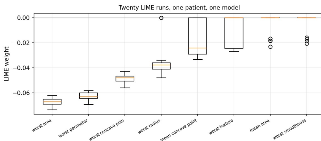
Figure. Twenty LIME runs for one patient with twenty seeds. Each box holds the twenty weights of one measurement, and a weight of 0 means that the run did not select it. Several features enter the top six in some runs and not in others.
