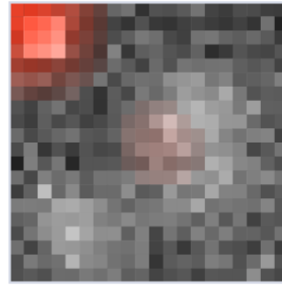
occlusion map
