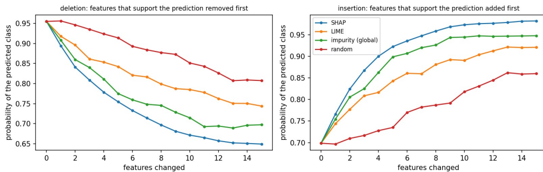
Figure. Mean deletion and insertion curves of four methods on 20 cases of the tumour data.
