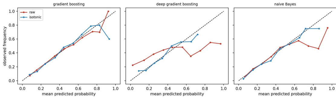
Figure. Reliability diagrams of three credit models on the 1200 test applicants, before recalibration (raw) and after isotonic recalibration. The dashed diagonal marks perfect calibration.
