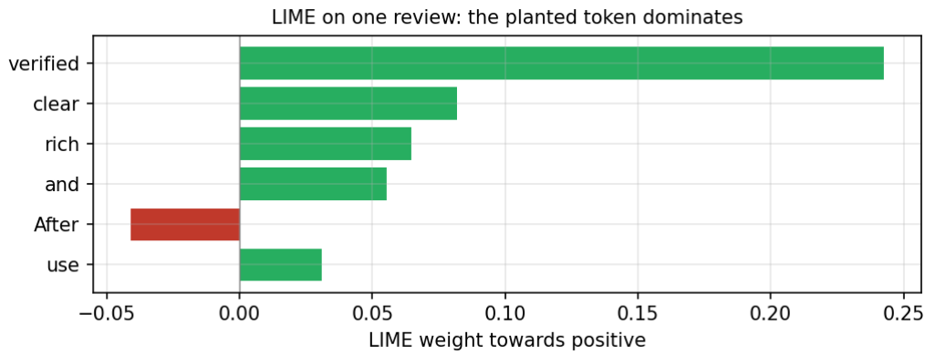
Figure. LIME weights for one review of the test data. The token verified carries no sentiment and has the largest weight.
