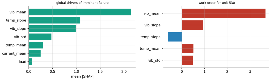
Figure. Left: the mean absolute SHAP value of each feature over the test windows, the global drivers of imminent failure. Right: the five largest SHAP values behind one work order. Red pushes towards failure and blue away from it.
