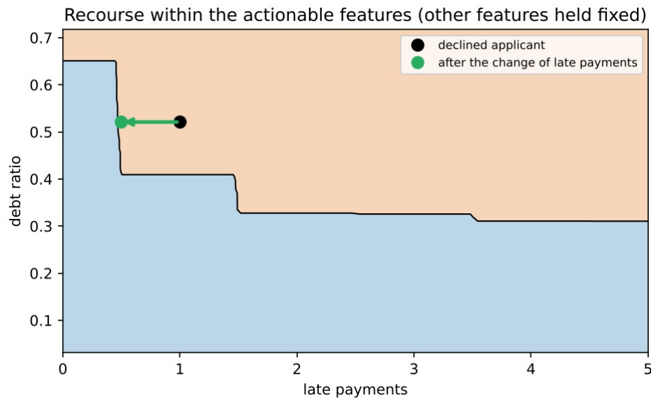
Figure. Applicant 1712 in the plane of late payments and debt ratio, with the other three features held at the values of the applicant. Orange is declined, blue is approved, and the black line is the decision boundary. The green arrow is the change of the statement.
