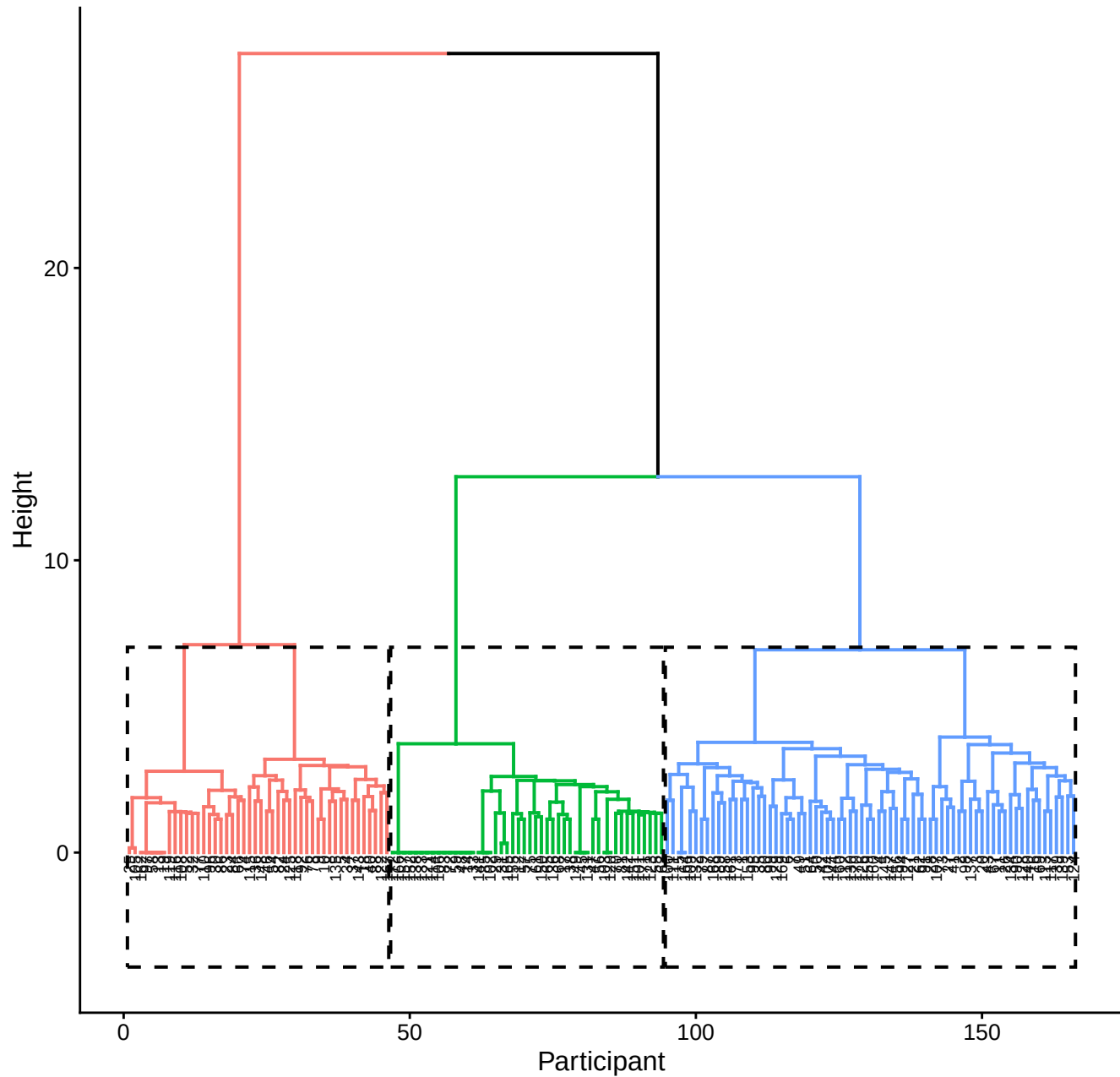
Hierarchical Clustering of Participants
