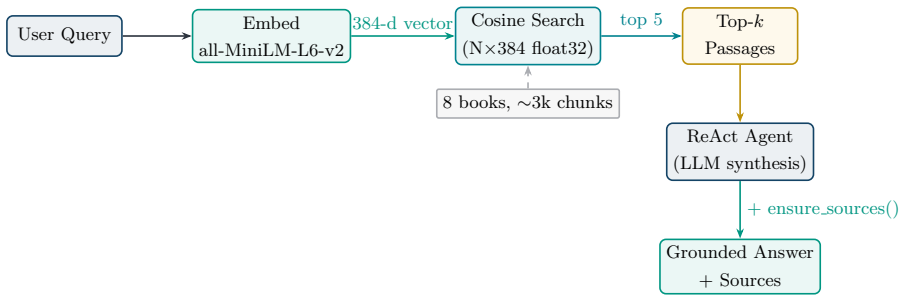
Fig. 6 RAG pipeline of the fitness specialist. The user query is embedded locally, compared against the normalised chunk vectors via dot product, and the top- k passages are fed to the ReAct agent for synthesis. The ensure_sources() step guarantees that book citations survive the orchestrator’s synthesis.
