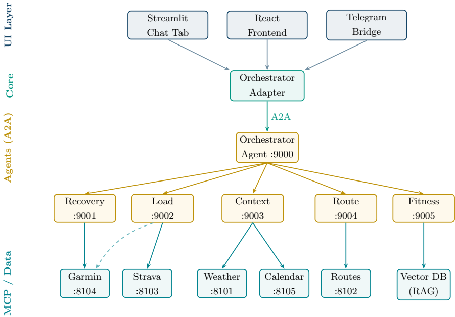
Fig. 3 Training Copilot system architecture. Solid arrows indicate primary communication paths; dashed arrows indicate secondary/fallback paths. Agents communicate via A2A; specialists access data via scoped MCP connections.
