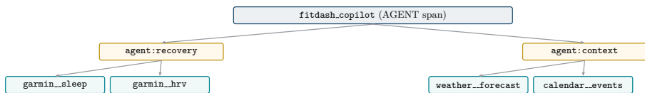
Fig. 8 Reconstructed span tree in the evaluation trace. Agent and tool spans are rebuilt from the Copilot’s trace dict and nested under the root evaluation span. Each tool span carries four custom attributes: fitdash.tool (name), fitdash.tool_ok (success), fitdash.tool_error (message), and fitdash.duration_ms (latency).
