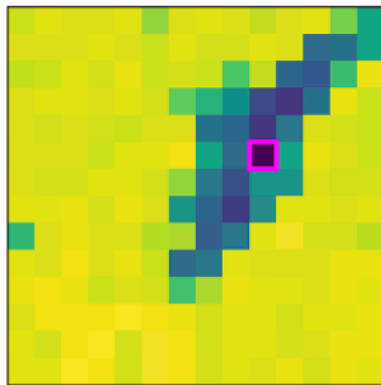
Encoder (t)
