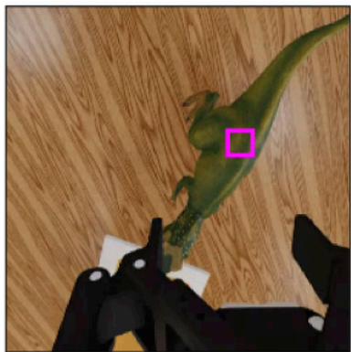
Frame (t)
