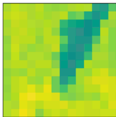
Predictor (t+1)
