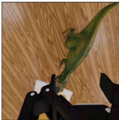
Frame (t+1)
