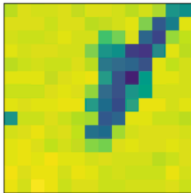
Encoder (t+1)
