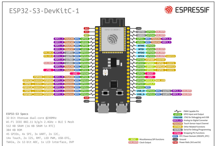
Fig. 2. ESP32-S3 Pinout.
