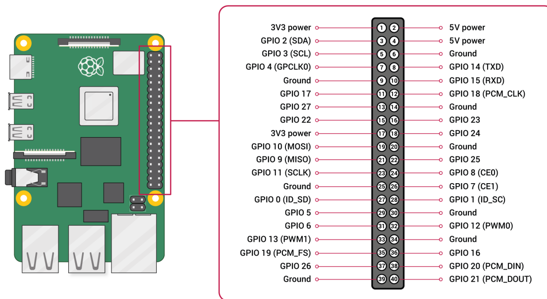
Figura 1: Pinout de Raspberry Pi 4.
