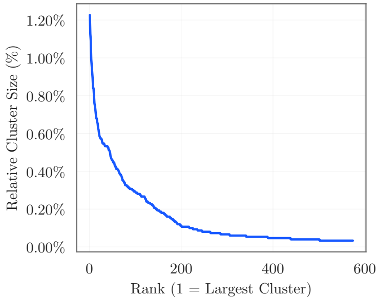
Rank-Size
