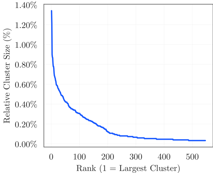
Rank-Size
