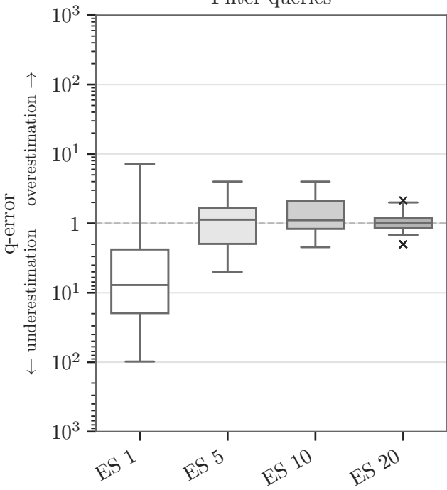
Filter queries
