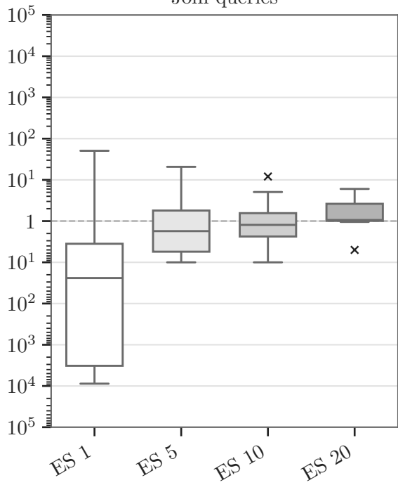
Join queries
