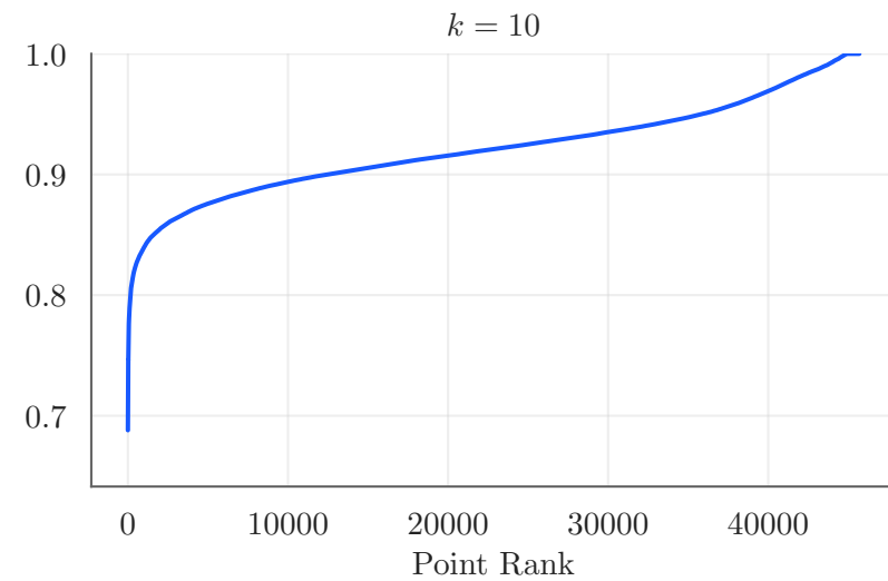
Arts_Crafts_and_Sewing_raw_5core / features_json_embeddings_google_siglip2_base_patch16_224 sorted similarities
