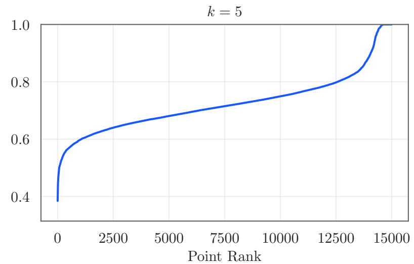
Arts_Crafts_and_Sewing_raw_5core / description_json_embeddings_qwen_qwen3_embedding_0.6b sorted similarities
