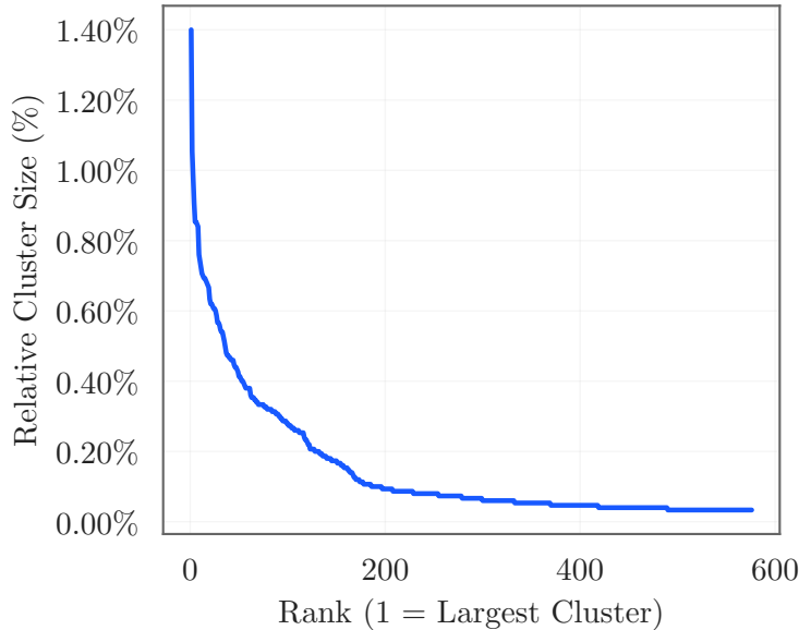
Rank-Size
