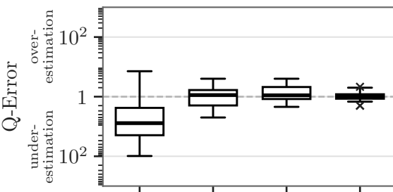
Filter Queries
