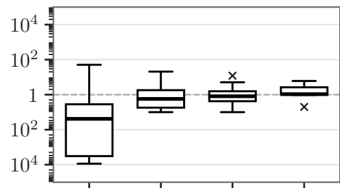
Join Queries
