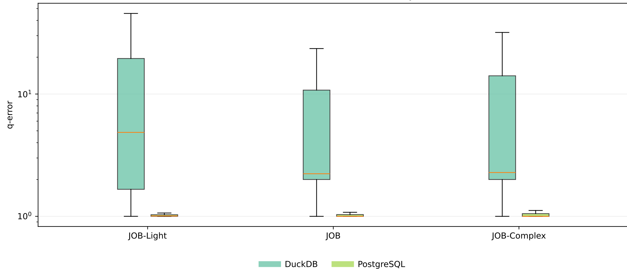
Balanced 200K Base-Selection Cardinality Q-Error
