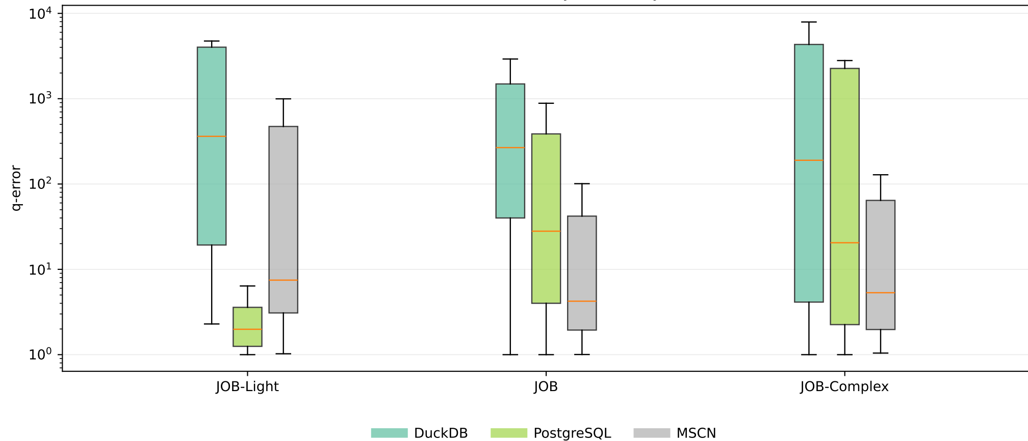
Balanced 200K Full-Query Cardinality Q-Error
