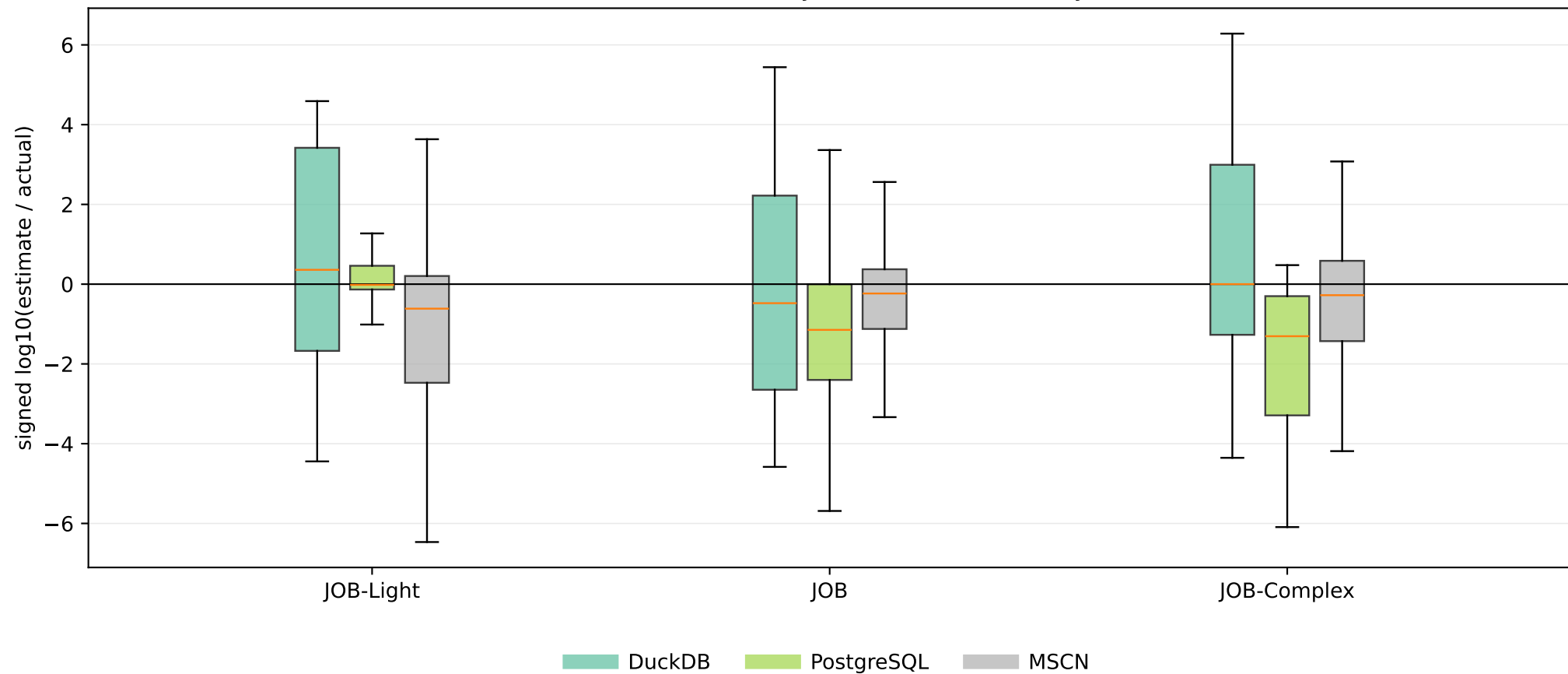
Balanced 200K Full-Query Directional Cardinality Error
