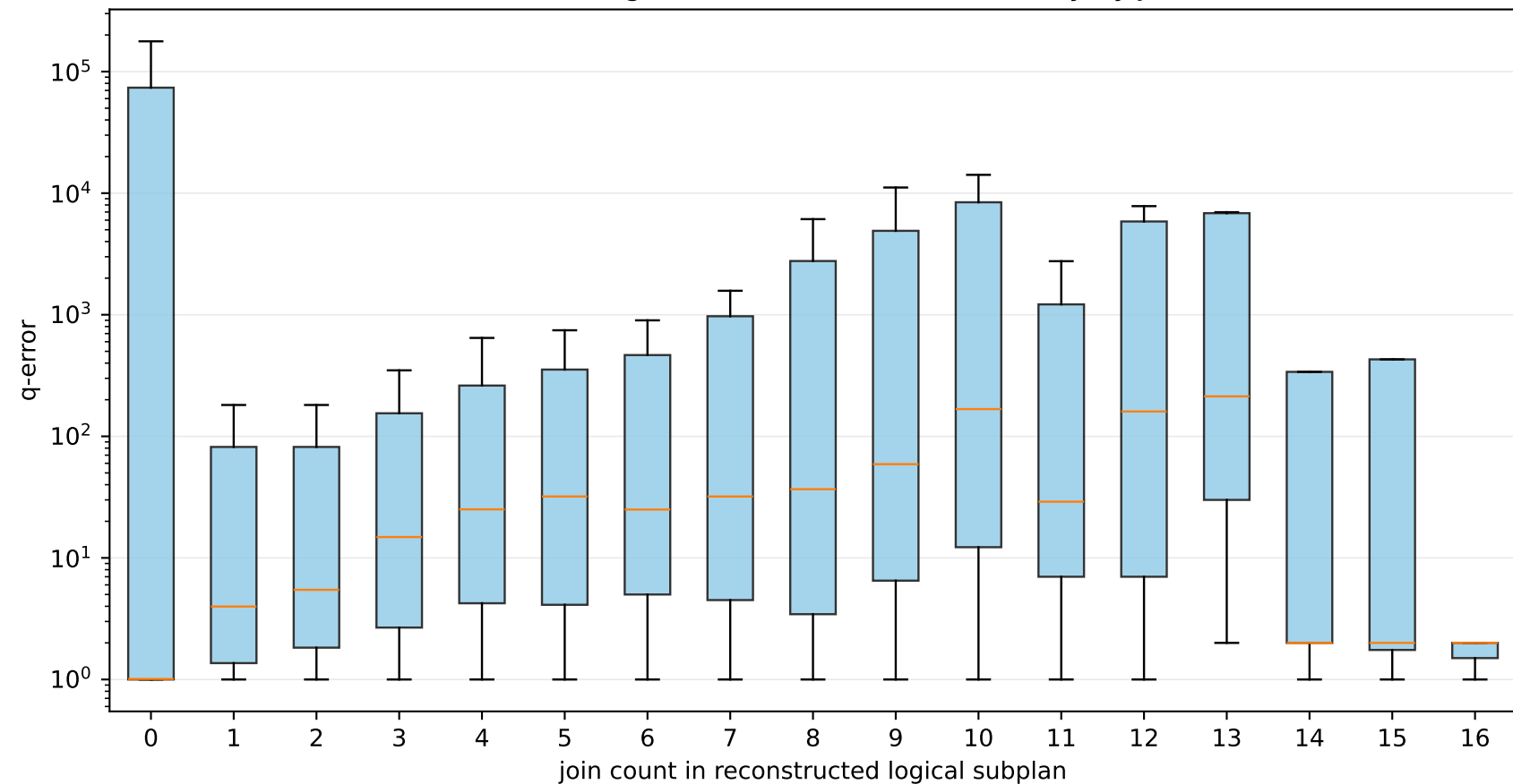
Balanced 200K PostgreSQL Intermediate Cardinality by Join Count
