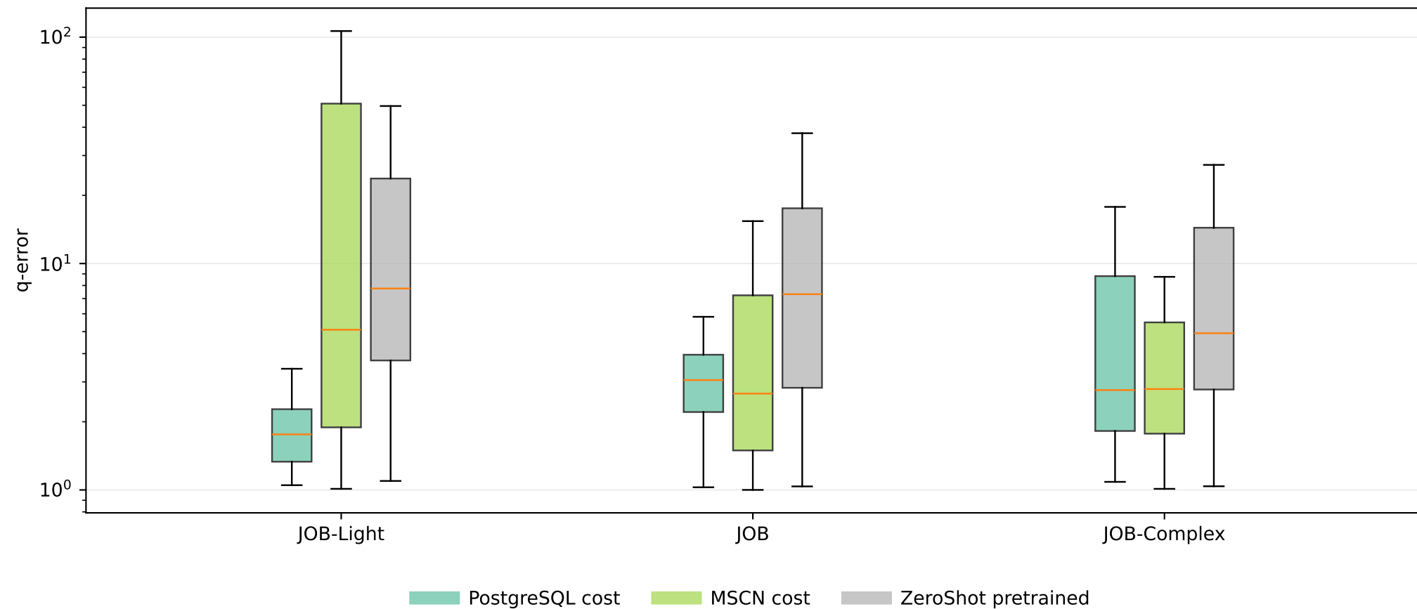
Balanced 200K Selected-Plan Cost/Runtime Q-Error
