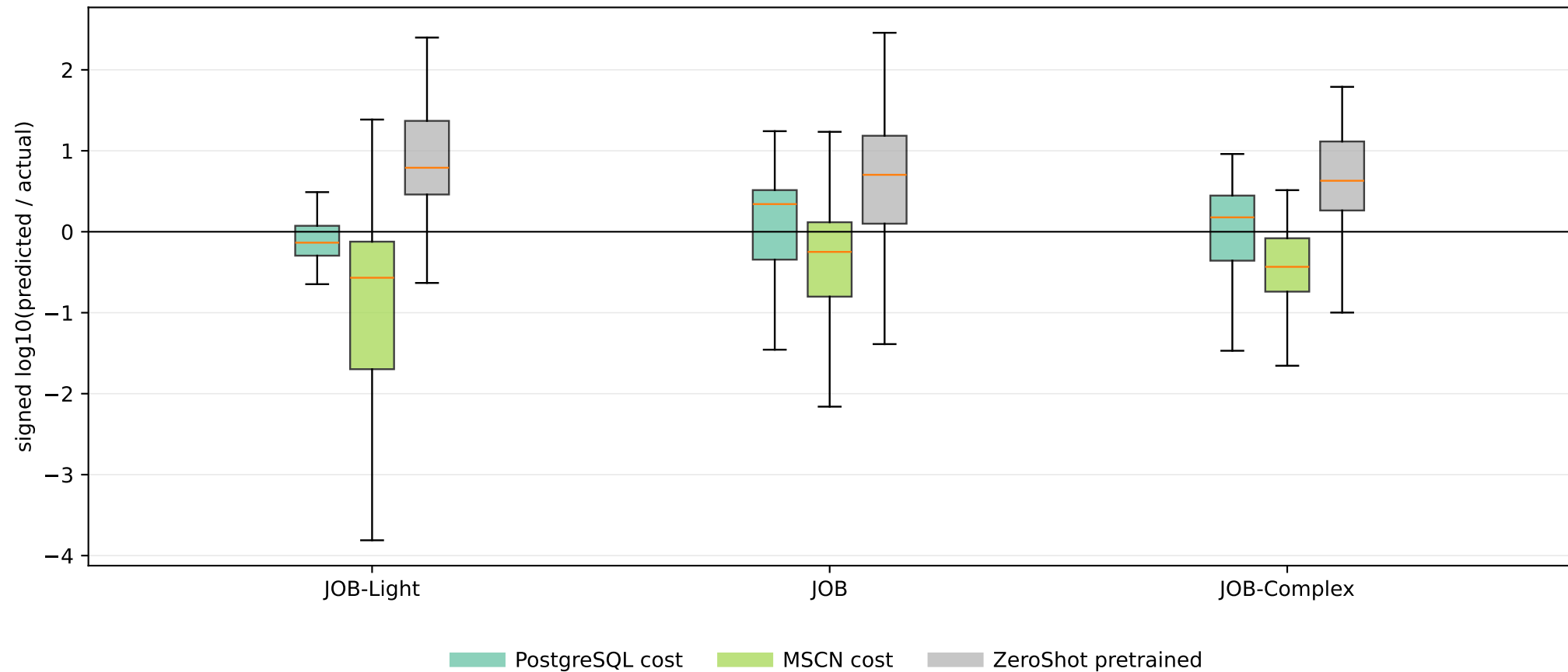
Balanced 200K Selected-Plan Directional Cost/Runtime Error
