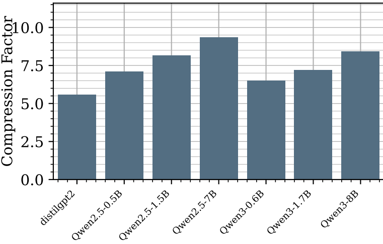
Wikipedia
