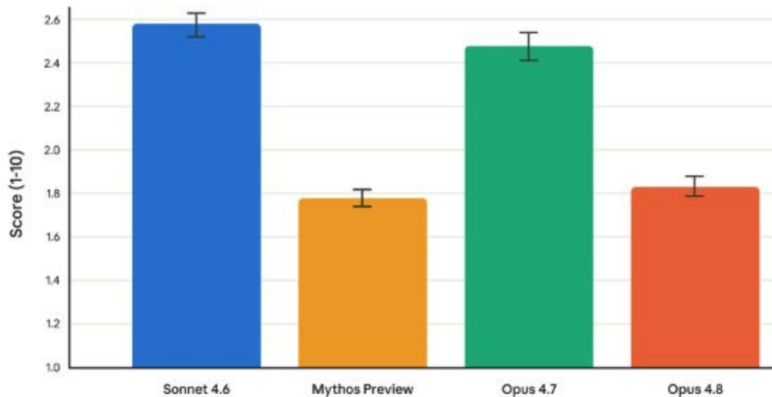
Misaligned behavior
