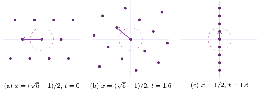
FIGURE 11. The grid g_t \Lambda_x near the origin, with a shortest non-zero vector drawn as an arrow and a disk of radius 0.6 dashed. The flow stretches the grid horizontally by e^t and squeezes it vertically by e^{-t} . For the badly approximable number x = (\sqrt{5} - 1)/2 , in (a) and (b), the grid is sheared but no non-zero point ever comes close to the origin, so the orbit stays bounded. For the rational number x = 1/2 , in (c), the points (0, 2qe^{-t}) with q \in \mathbb{Z} crowd towards the origin, and the orbit goes into the cusp.
