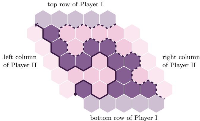
FIGURE 14. The no-draw argument on a full 5 \times 5 board (see Theorem 17.1). The stones of Player I are plum and those of Player II are pink; the paler cells are the extra rows and columns. The walk starts at the lower left corner, between the two colours, and follows the edges that separate plum from pink. It cannot stop or turn back, so it leaves the board at another corner, and the plum stones along its right side form a chain from bottom to top. The dashed line is the walk that starts at the lower right corner.
