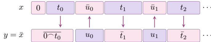
FIGURE 13. Stealing Player II's strategy in \text{Ul}(\mathcal{U}) . Lavender blocks are answers of the strategy \tau , blush blocks are moves of Player I, and each arrow copies an answer of \tau in one game, flipped, as a move of Player I in the other.
