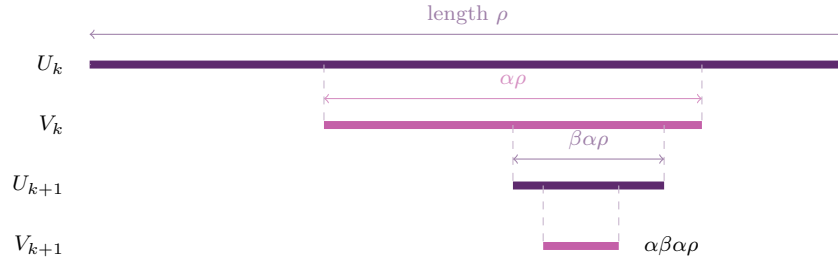
FIGURE 10. Two rounds of Schmidt's (\alpha, \beta) -game on the line, drawn with \alpha = \frac{1}{2} and \beta = \frac{2}{5} . Player I (plum) and Player II (pink) take turns choosing closed intervals, each inside the previous one, and the lengths are prescribed: Player II shrinks by the factor \alpha , Player I by the factor \beta . Only the positions of the intervals are up to the players.
