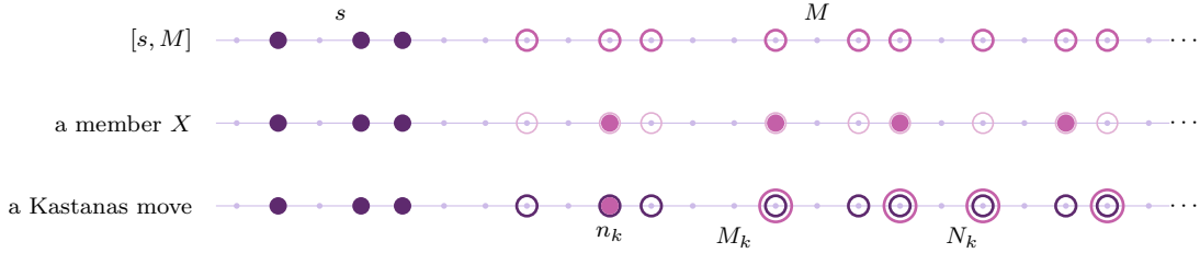
FIGURE 12. The Ellentuck topology on [\omega]^\omega . Top: a basic open set [s, M] is given by a finite stem s (filled plum) and an infinite set M above it (circles). Middle: a member of [s, M] is the stem together with an infinite subset of M (filled pink). Bottom: one round of the Kastanas game after the stem: Player I offers an infinite set M_k (plum circles), and Player II commits to one element n_k \in M_k and keeps an infinite set N_k \subseteq M_k above it (pink circles) for the rest of the play.
