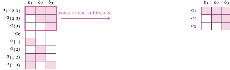
FIGURE 5.1. The proof of Proposition 5.1.2 for n = 3 . Left: shattered tuples b_1, b_2, b_3 , with one row a_S for each S \subseteq \{1, 2, 3\} and a pink cell where \varphi(a_S, b_j) holds. Right: the three rows indexed by the suffixes S_1 = \{1, 2, 3\} , S_2 = \{2, 3\} and S_3 = \{3\} (framed) form the staircase of a 3-ladder (compare Figure 1.1). A ladder uses only n of the 2^n rows, which is why the order property does not give the independence property (Example 5.1.3).
