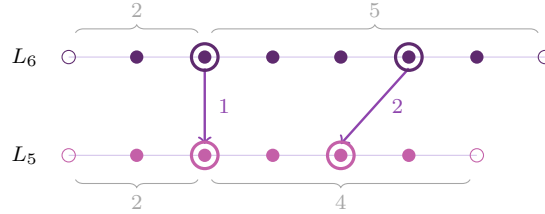
FIGURE 21. A play of \text{EF}_2(L_6, L_5) , with the imaginary elements below and above each order drawn as open circles. After round 1 the gaps are 2 and 5 in L_6 and 2 and 4 in L_5 : equal, or both at least 2^{2-1} = 2 , as the invariant requires. In round 2 Player I chooses an element in the long gap of L_6 , and Player II answers in the corresponding gap of L_5 . The chosen elements are in the same order in both structures, so Player II wins.
