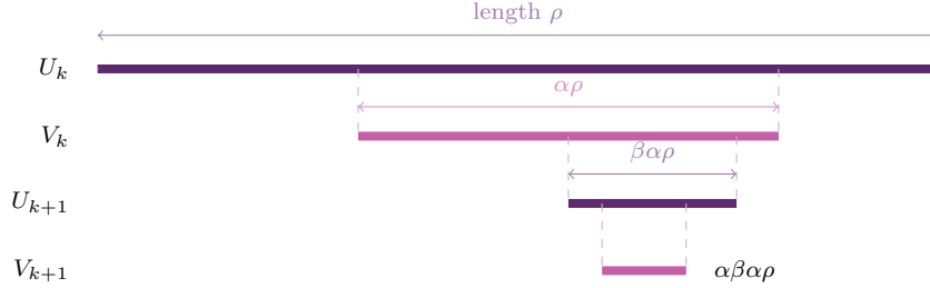
FIGURE 12. Two rounds of Schmidt's (\alpha, \beta) -game on the line, drawn with \alpha = \frac{1}{2} and \beta = \frac{2}{5} . Player I (plum) and Player II (pink) take turns choosing closed intervals, each inside the previous one, and the lengths are prescribed: Player II shrinks by the factor \alpha , Player I by the factor \beta . Only the positions of the intervals are up to the players.
