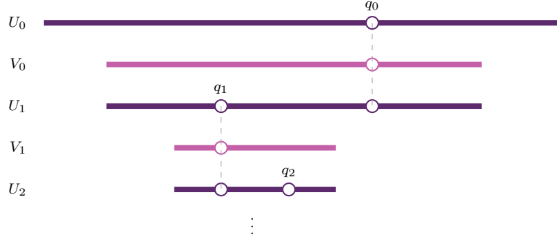
FIGURE 6. Player I wins \text{BM}(\mathbb{Q}) (see Example 3.2(1)). The moves of Player I are drawn in plum and those of Player II in pink, as intervals of rationals. At step n Player I removes the rational q_n (a hole), and a hole, once made, persists in every later set. Every rational is removed at some step, so the sets have no point in common.
