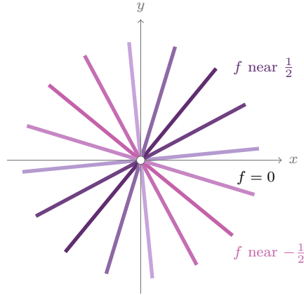
FIGURE 14. The function f(x, y) = xy/(x^2 + y^2) , with f(0, 0) = 0 , is constant on each ray from the origin, where it equals \frac{1}{2} \sin 2\theta ; the colour shows the value. On the axes f vanishes, so f is continuous in each variable separately. Every neighbourhood of the origin contains all the values between -\frac{1}{2} and \frac{1}{2} , so f is not jointly continuous there.
