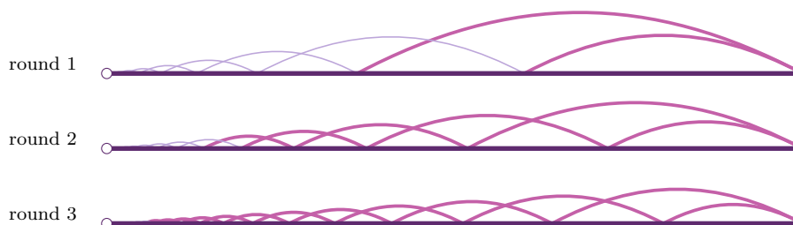
FIGURE 17. The Menger game on the half-open interval X = (0, 4] . In each round Player I chooses an open cover of X , drawn as arcs, here by intervals that accumulate at 0; Player II keeps finitely many of them (pink). No single round covers X , since finitely many of the intervals miss a neighbourhood of 0. But X is \sigma -compact, and Player II covers a larger compact piece of X in each round, so that her choices together cover all of X .
