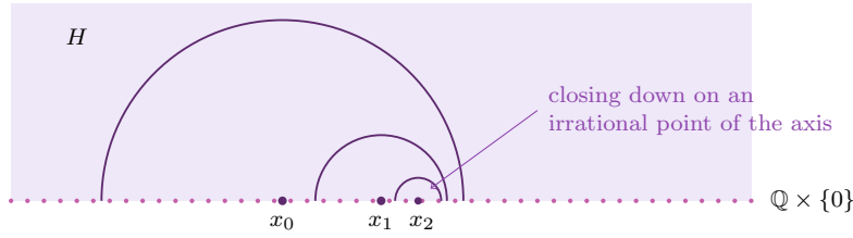
FIGURE 9. Player I wins \text{Ch}(X) for the space X of Remark 4.6. He plays rational points of the axis, with small balls of X about them, inside the previous answer of Player II, and avoids one more rational each time. The balls close down on a point of the axis that is not rational, hence not in X .
