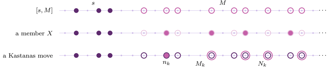
FIGURE 15. The Ellentuck topology on [\omega]^\omega . Top: a basic open set [s, M] is given by a finite stem s (filled plum) and an infinite set M above it (circles). Middle: a member of [s, M] is the stem together with an infinite subset of M (filled pink). Bottom: one round of the Kastanas game after the stem: Player I offers an infinite set M_k (plum circles), and Player II commits to one element n_k \in M_k and keeps an infinite set N_k \subseteq M_k above it (pink circles) for the rest of the play.
