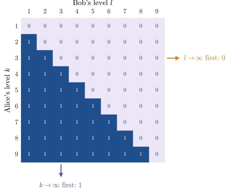
FIGURE 2. The energy comparison of two oscillators: the value \varphi(e_k, f_l) is 1 when Alice's level k exceeds Bob's level l and 0 otherwise. Every row tends to 0 as l \rightarrow \infty , and every column tends to 1 as k \rightarrow \infty , so the two iterated limits are 0 and 1.
