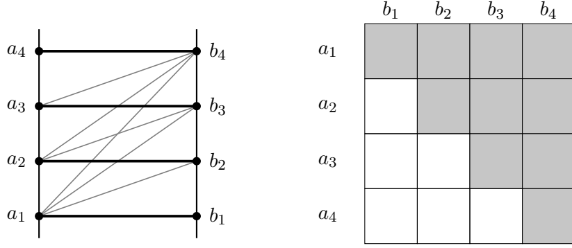
FIGURE 1.1. A 4-ladder. Left: the elements a_i and b_j are joined when \varphi(a_i, b_j) holds, i.e. when i \leq j . The pairs (a_i, b_i) are the rungs (thick), and each a_i also reaches every b_j with j > i (gray). Right: the truth table of \varphi(a_i, b_j) , with shaded cells where \varphi holds. The table is a staircase, which is why an n -ladder is also called a half-graph .
