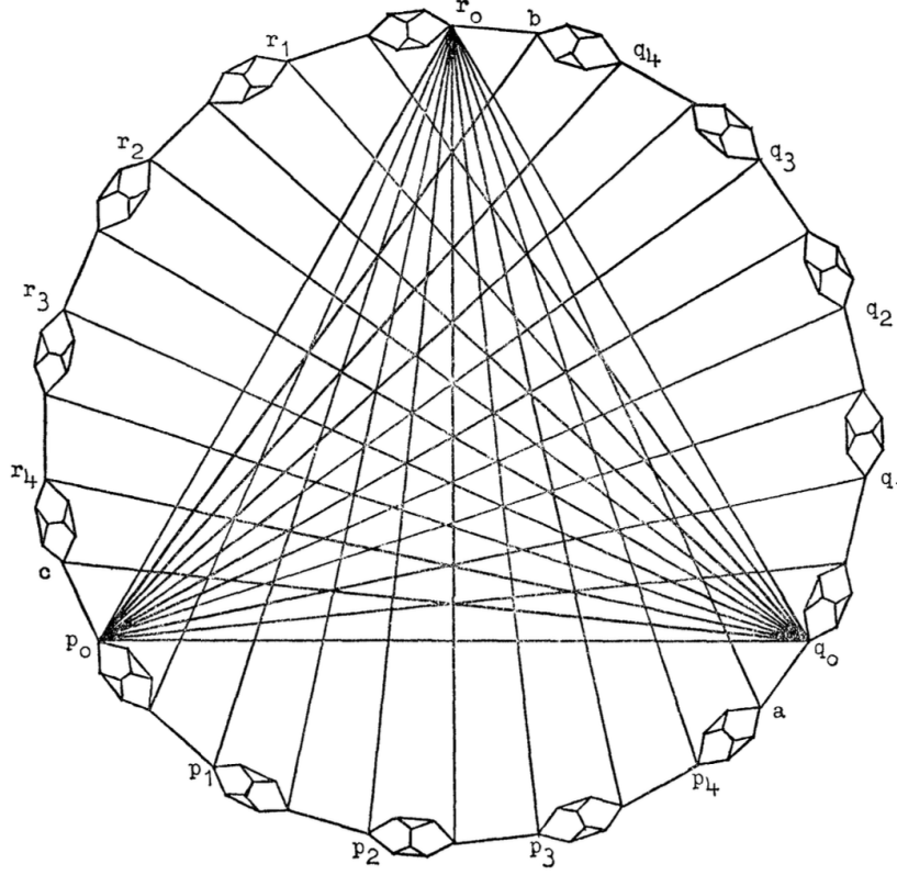
FIGURE 1. The graph \Gamma_2 of Kochen and Specker's 1967 paper [KS67, p. 69], whose 117 vertices are the vectors of their original proof; two vertices are joined by an edge when the corresponding vectors are orthogonal. The vertices are the points on the rim, after identifying p_0 with a , q_0 with b , and r_0 with c ; each of the fifteen small gadgets on the rim is a copy of their ten-vertex graph \Gamma_1 .
