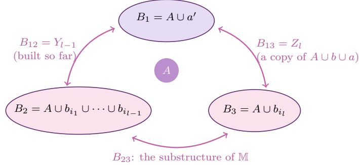
FIGURE 5.9. The inductive step in the proof of Theorem 5.5.9(1). The fresh copy a' of a has already been joined to the first l - 1 terms (the structure Y_{l-1} ); it must now be joined to b_{i_l} as a is joined to b (the structure Z_l ), while the terms of the sequence keep the structure they have in \mathbb{M} . Disjoint 3-amalgamation over A glues the three prescriptions into Y_l . In the Rado graph nothing has to be glued, because every relation is binary and every graph is allowed.
