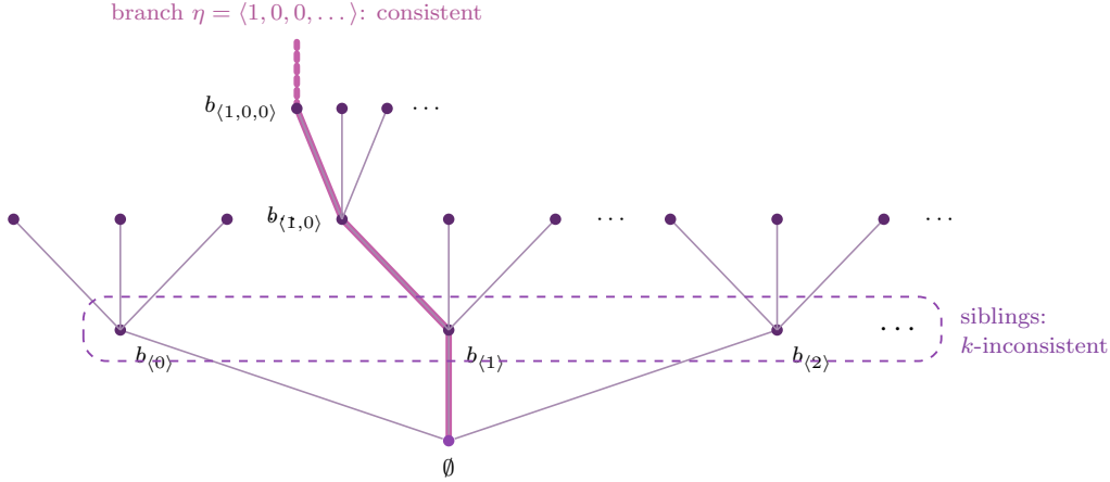
FIGURE 5.1. The k -tree property (see Definition 5.2.6). The tree grows upward; the node \sigma carries the parameter b_\sigma . Along every branch (pink) the formulas \varphi(x, b_{\eta|n}) have a common solution, while the formulas attached to the siblings of any node (framed for the successors of the root) are k -inconsistent: no k of them hold together.
