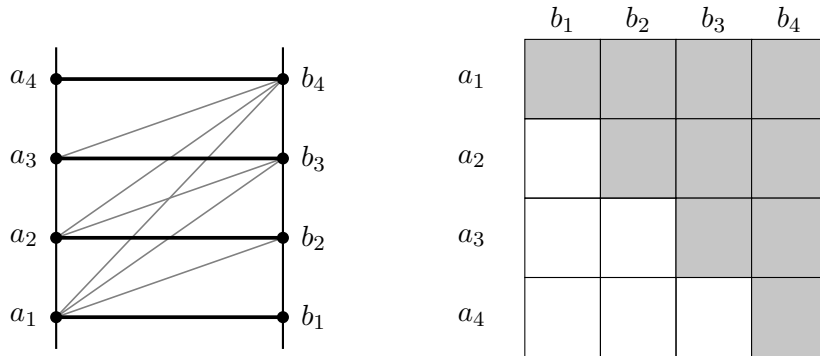
FIGURE 1. A 4-ladder. Left: a_i and b_j are joined when \varphi(a_i, b_j) holds, i.e. when i \leq j . The pairs (a_i, b_i) are the rungs (thick), and each a_i also reaches every b_j with j > i (gray). Right: the truth table of \varphi(a_i, b_j) , with shaded cells where \varphi holds. The table is a staircase, which is why an n -ladder is also called a half-graph .
