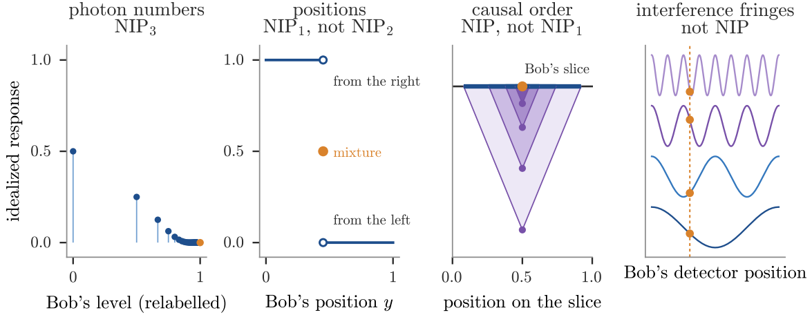
FIGURE 6. Pictures for parts (a), (b), (c) and (e) of Theorem 16.1. Photon numbers: a monotone response on the relabelled spectrum \{1 - \frac{1}{l+1}\} , whose points accumulate only at 1. Positions: a particle concentrating at a point from the right or from the left gives two idealized responses that differ only there, and their mixture gives the midpoint. Causal order: events closer and closer to Bob's time slice, whose light cones meet it in intervals shrinking to a single point. Fringes: at a single detector position, fringes of increasing wavenumber realize a prescribed pattern (shown here 1, 2, 4, 8; the proof uses 8^n ).
