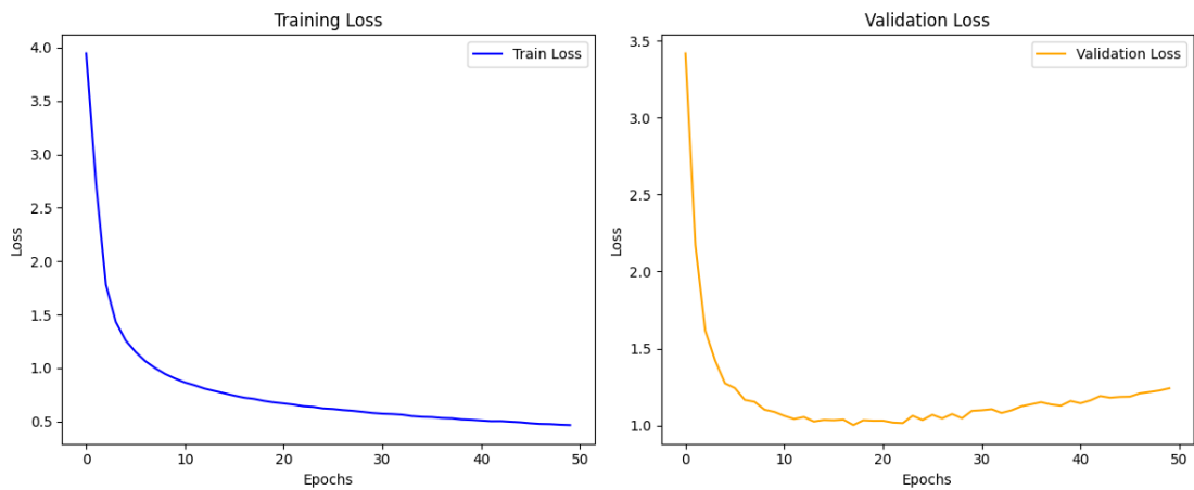
Figure 6-17 Training Loss vs Epochs (OCR)
