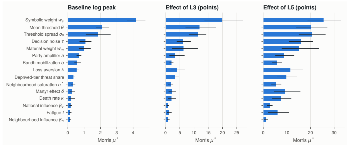
Figure 10: Morris \mu^* with 95% bootstrap intervals over trajectories, stylized specification.
