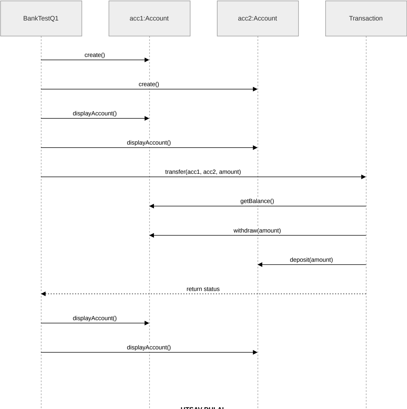
UTSAV DULAL Fig: SEQUENCE DIAGRAM
