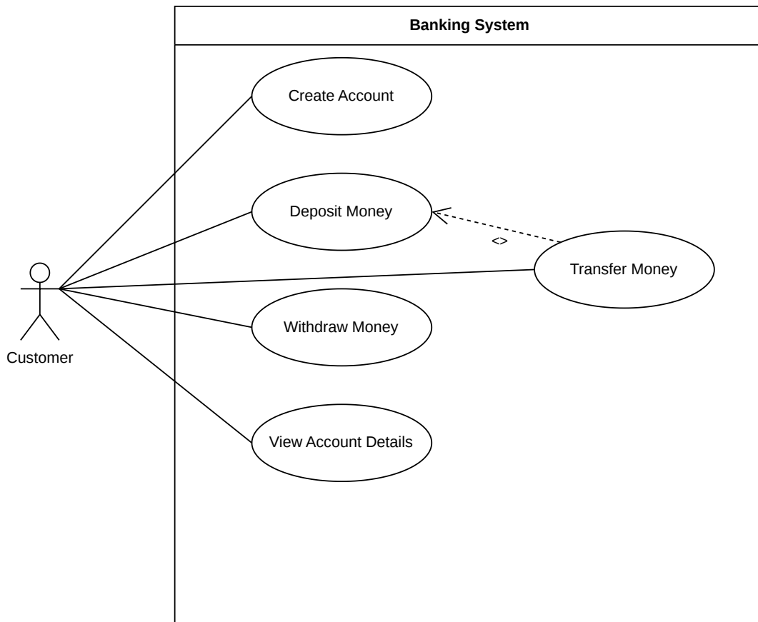
UTSAV DULAL Fig: USE CASE DIAGRAM
