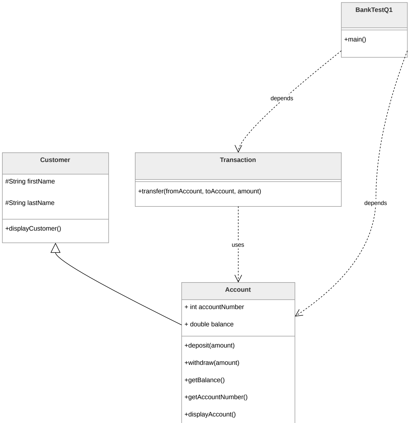
UTSAV DULAL Fig: CLASS DIAGRAM
