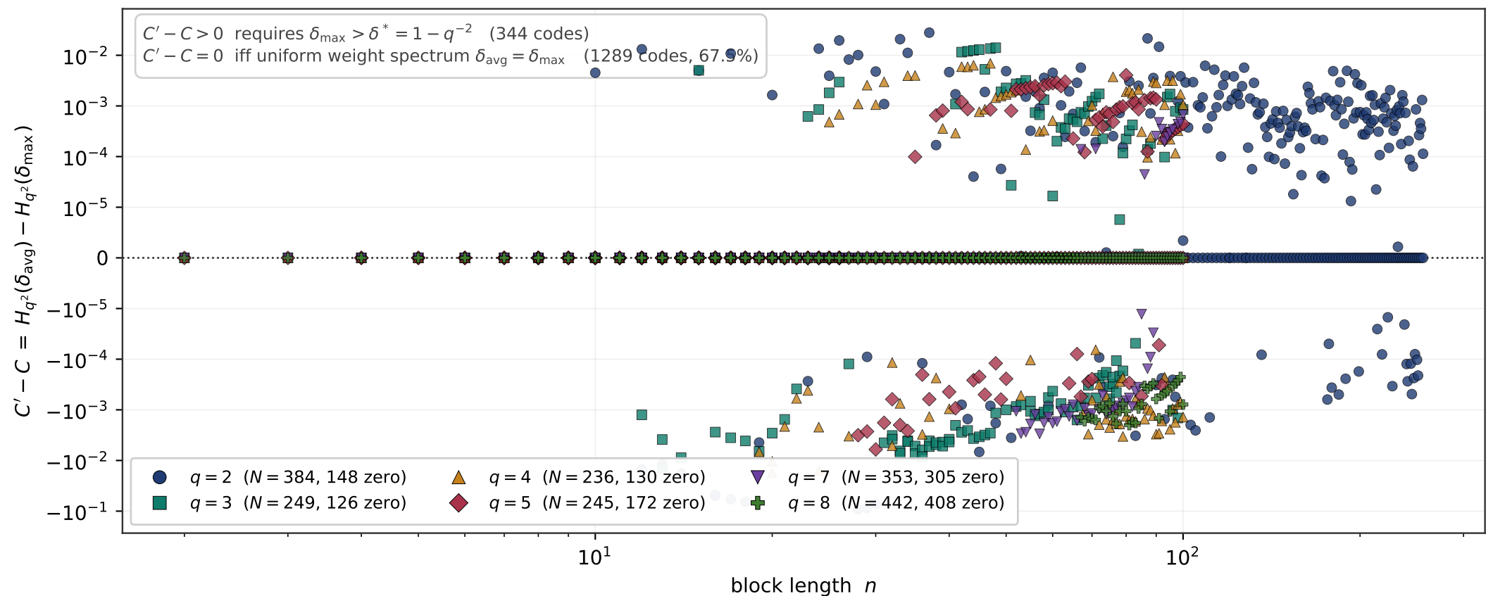
C' - C for semi-perfect quantum codes ( N = 1909 ; symlog scale, linear within \pm 1e - 05 )
