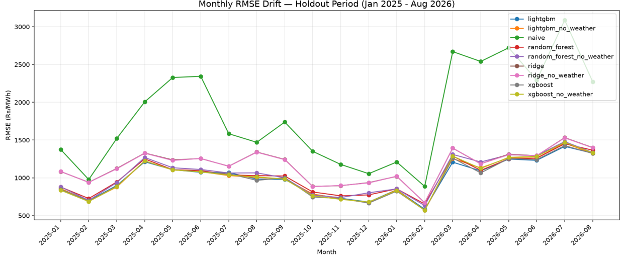
Figure 4: Monthly RMSE drift over the 20-month holdout (January 2025–August 2026). Learned models (clustered lines, lower band) remain stable while the naive weekly-persistence baseline (green) spikes during high-volatility spring months. Weather and no-weather variants of each model are visually indistinguishable, echoing Table 3.
